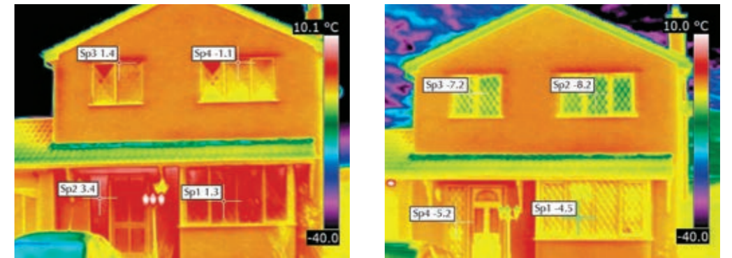
BEFORE and AFTER: The above thermal images clearly demonstrate the advantages of installing new energy efficient windows. The heat loss temperature of the living room window is 1.3°C before and -4.5°C after the new windows were fitted - a significant reduction.
